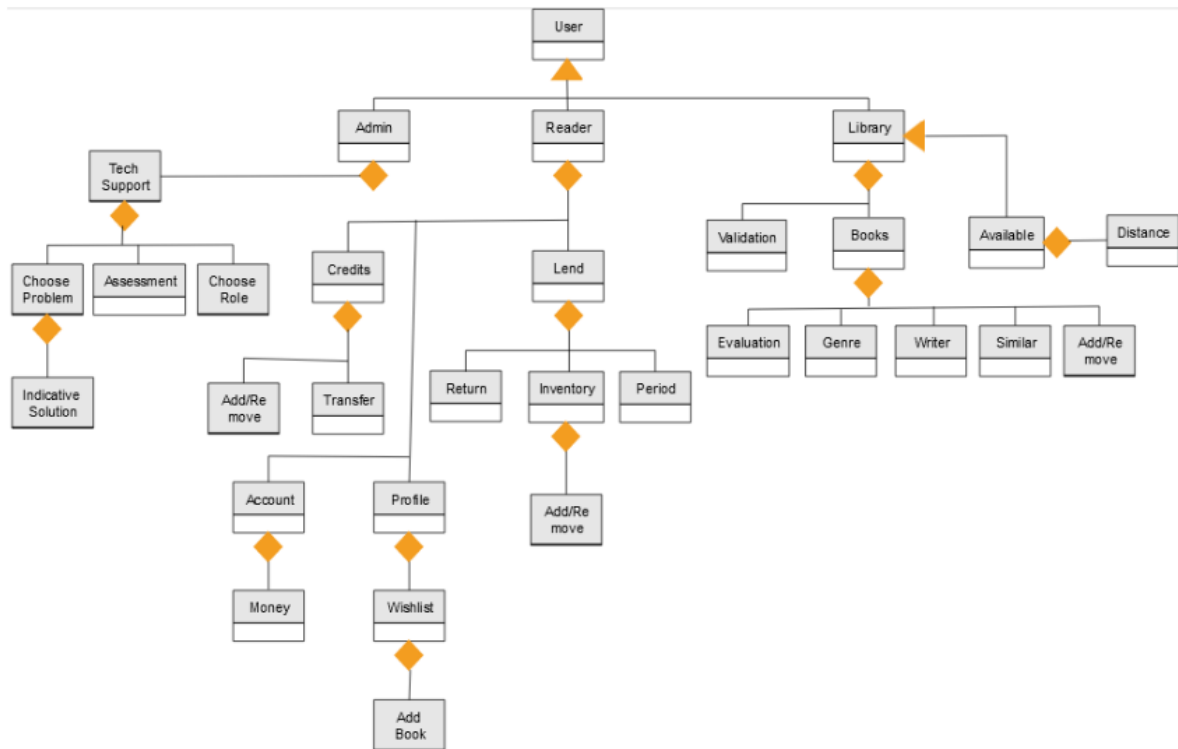
Figure 1: Schematic Diagram of the Domain Model
